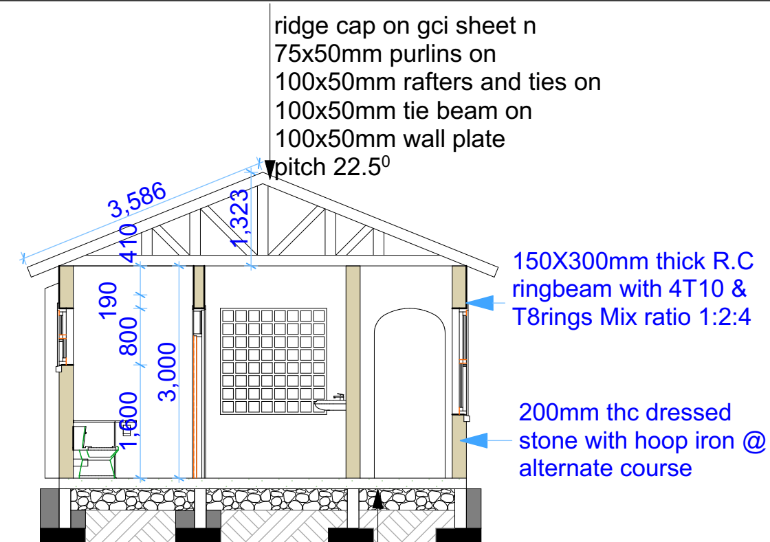
SECTION
