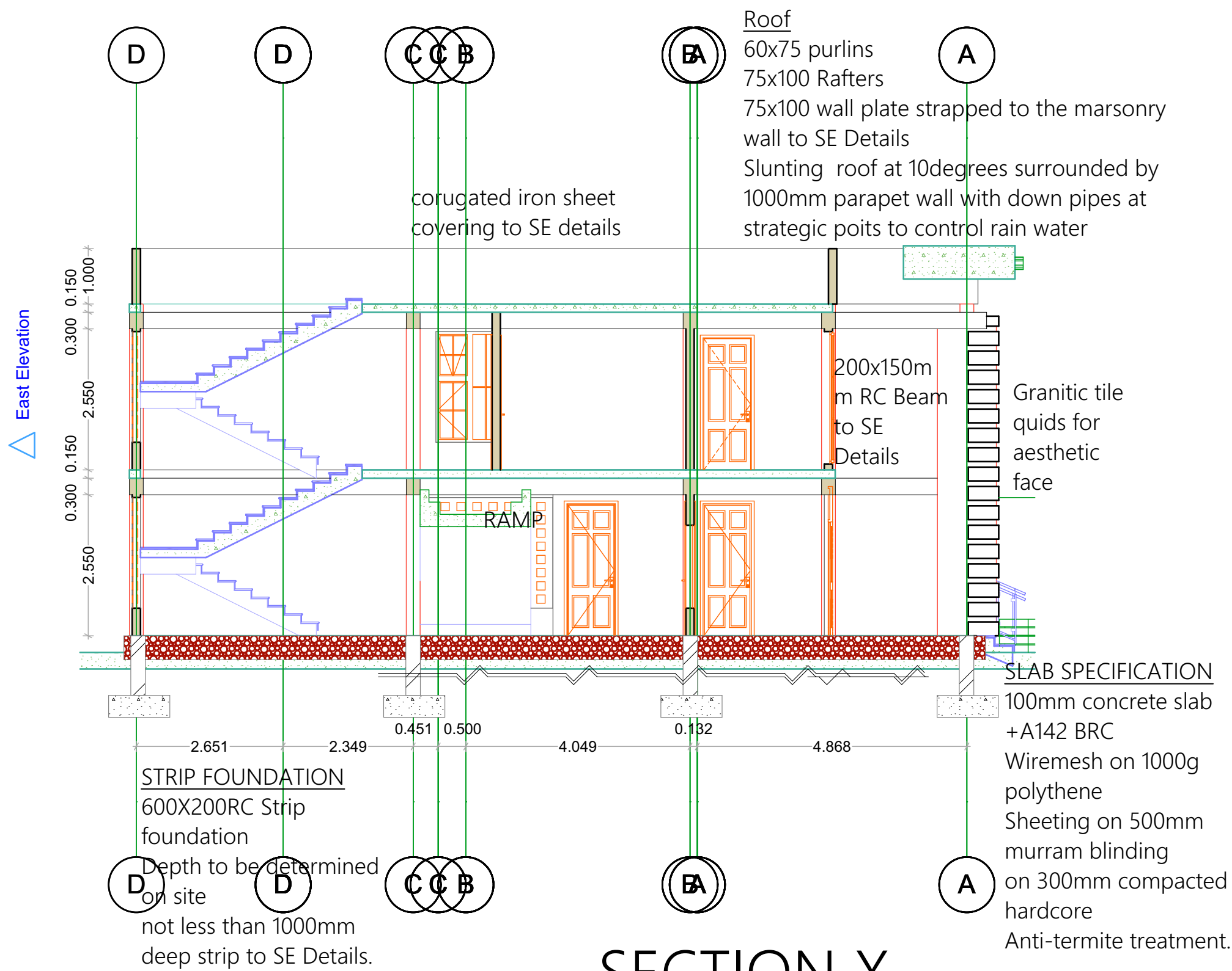
SECTION X
