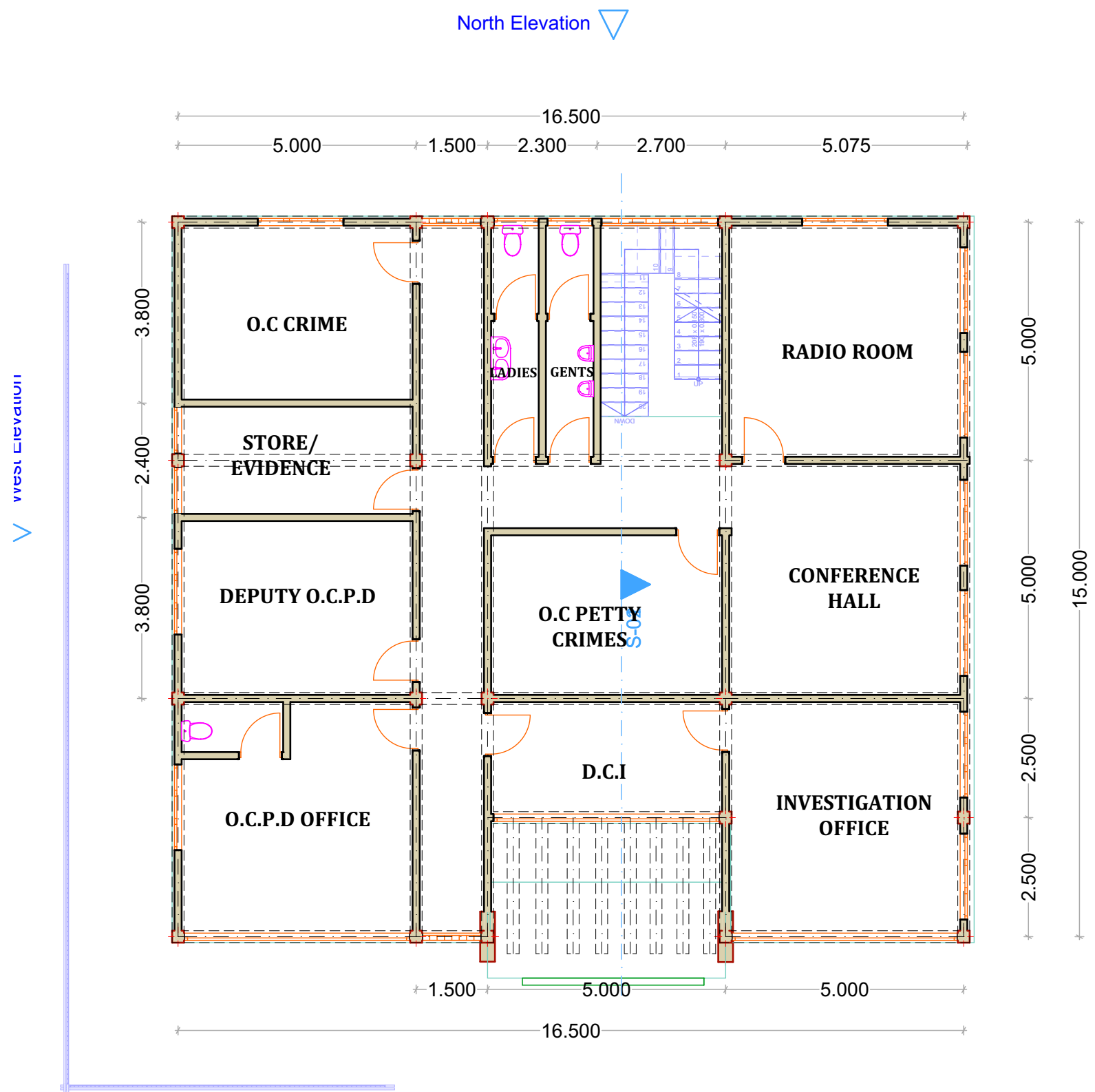
FIRST FLOOR
