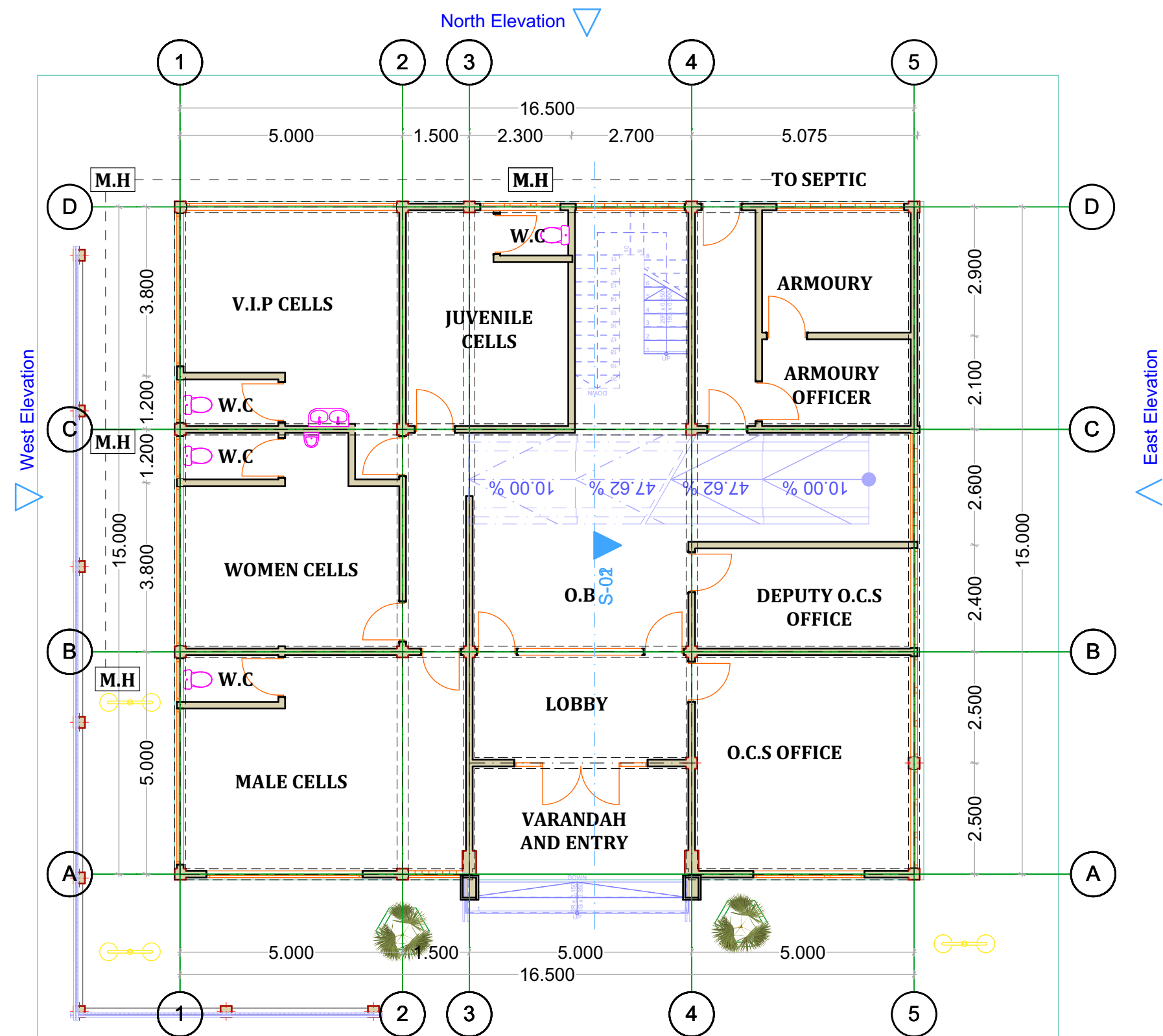
GROUND FLOORPLAN
