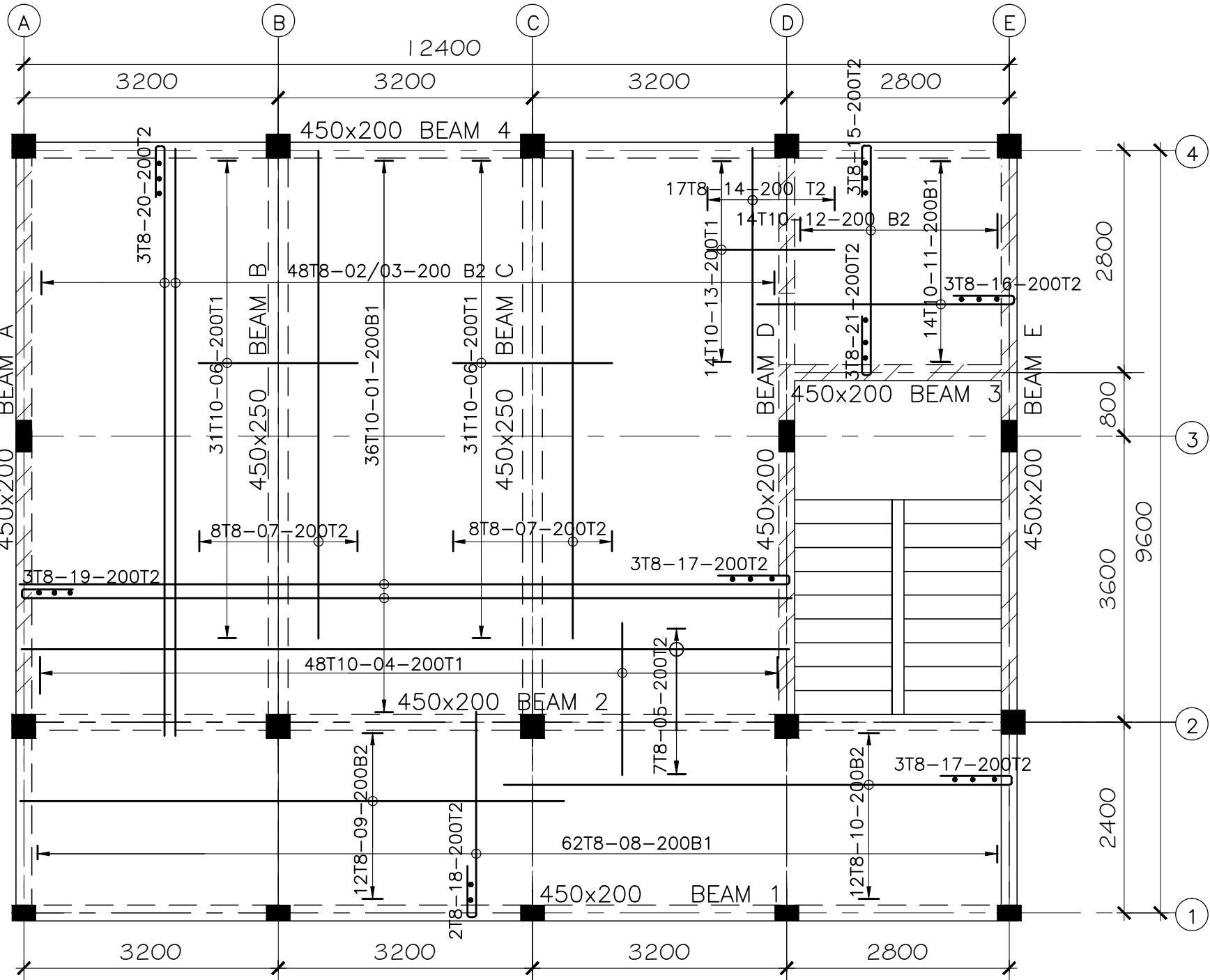
UPPER FLOOR, PART 375mm HOLLOW BLOCK SLAB & 150 mm THICK PART SOLID SLAB R.C LAYOUT & DETAILS
