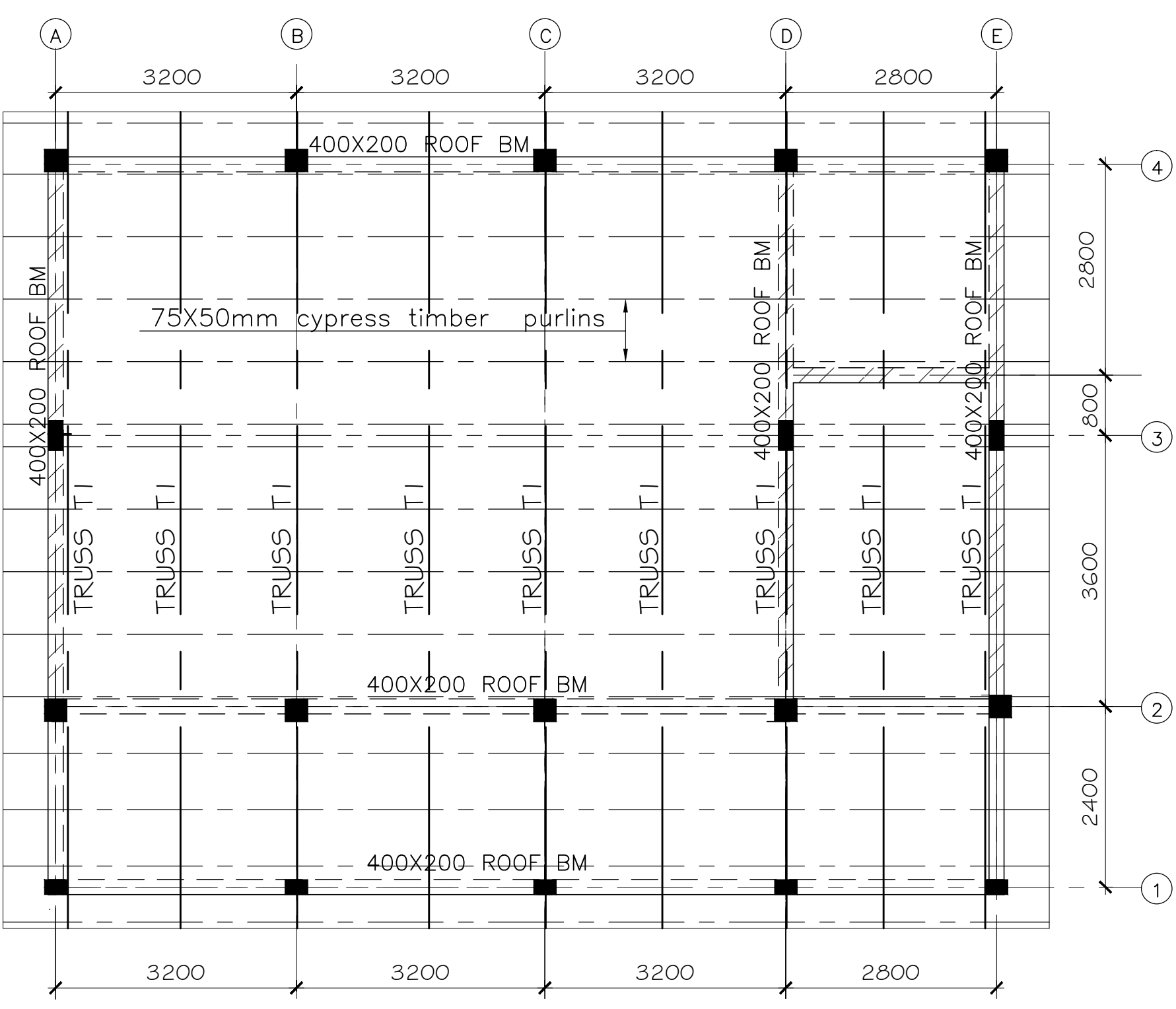
ROOF LAYOUT
