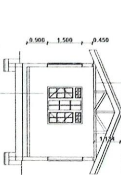
SECTION 01-01
