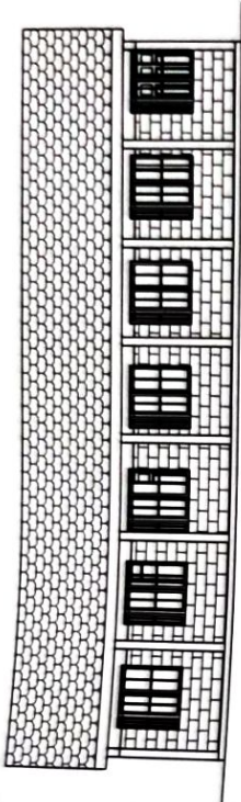
ELEVATION 03 SCALE 1:100
