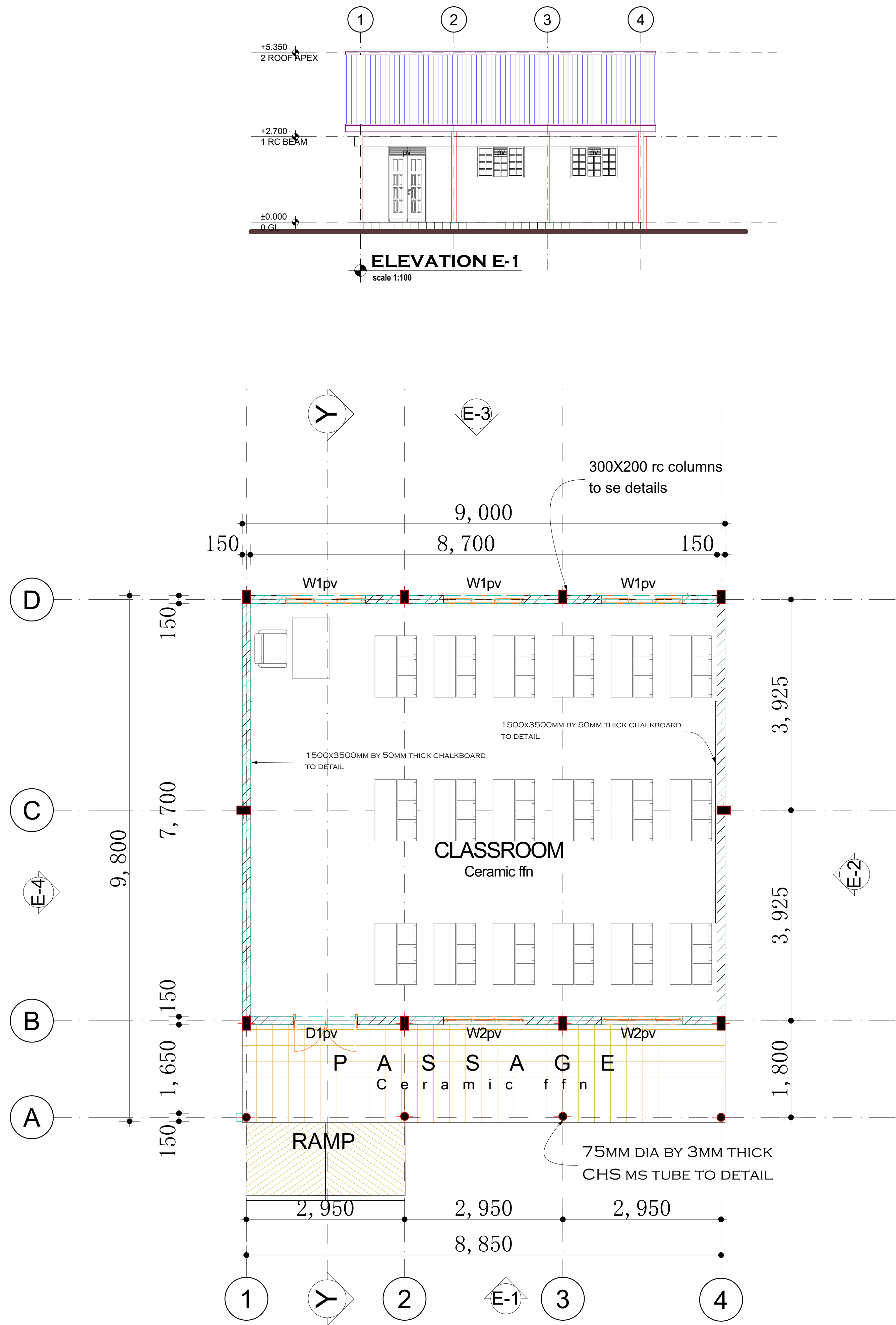
FLOOR PLAN SCALE 1:100
