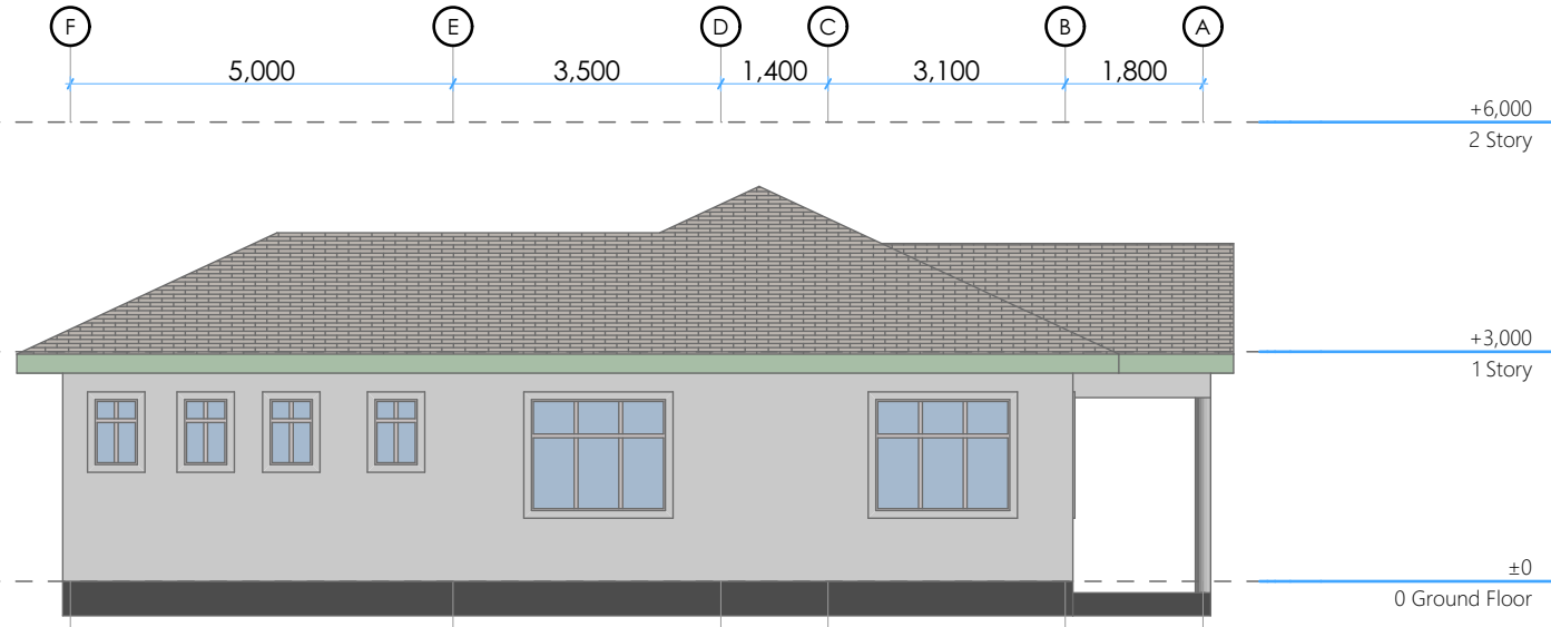
SIDE ELEVATION 04
