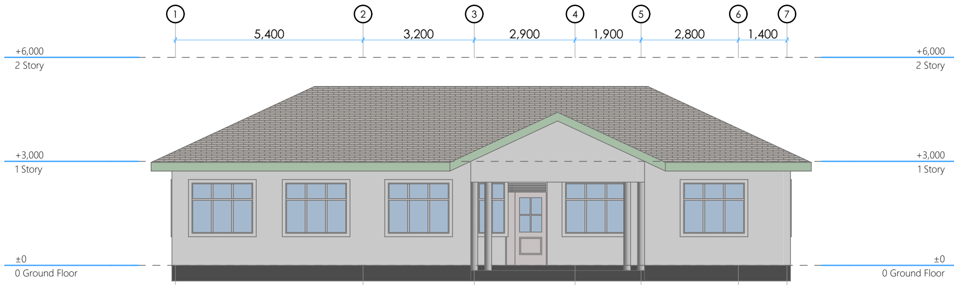
FRONT ELEVATION 01
