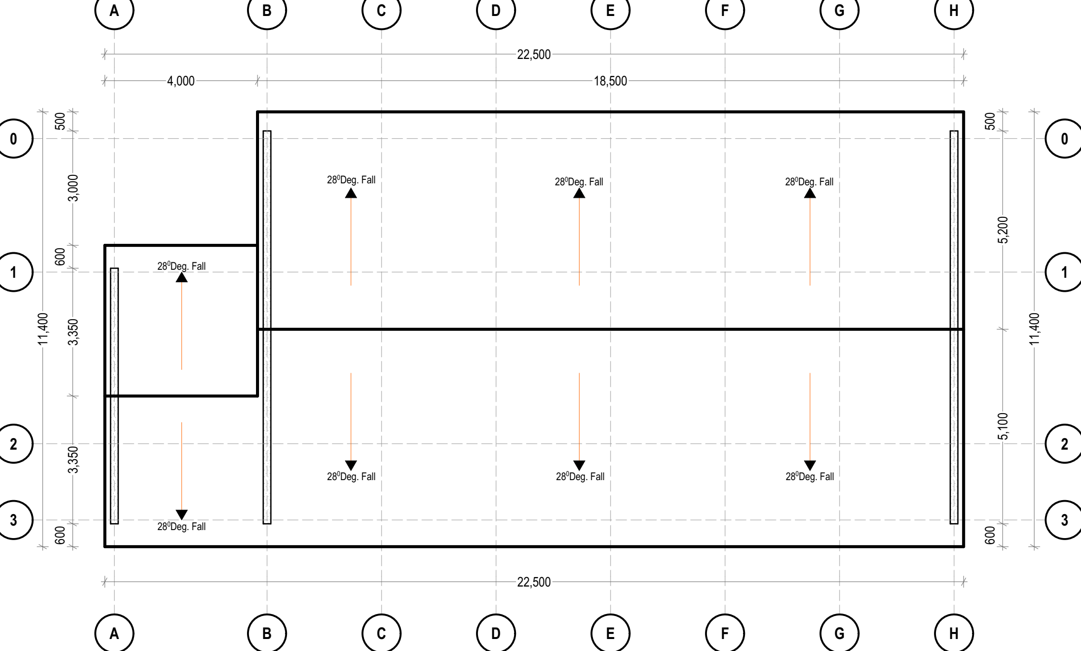
Roof Plan Layout SCALE 1:100
