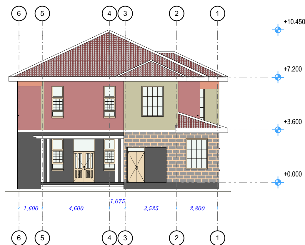
ELEVATION 02 SCALE 1:100
