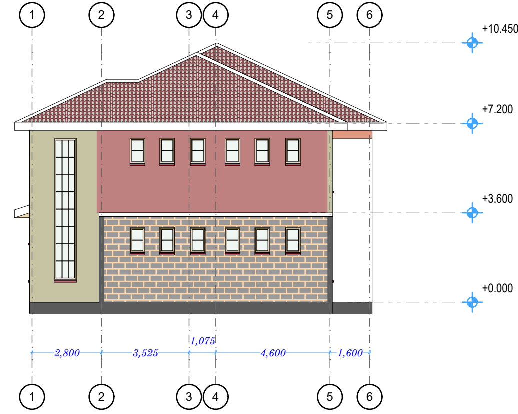
ELEVATION 04 SCALE 1:100
