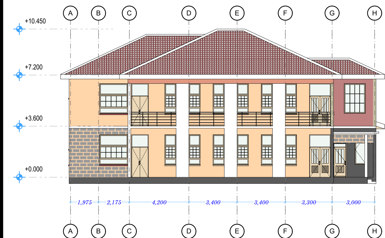
ELEVATION 03 SCALE 1:100
