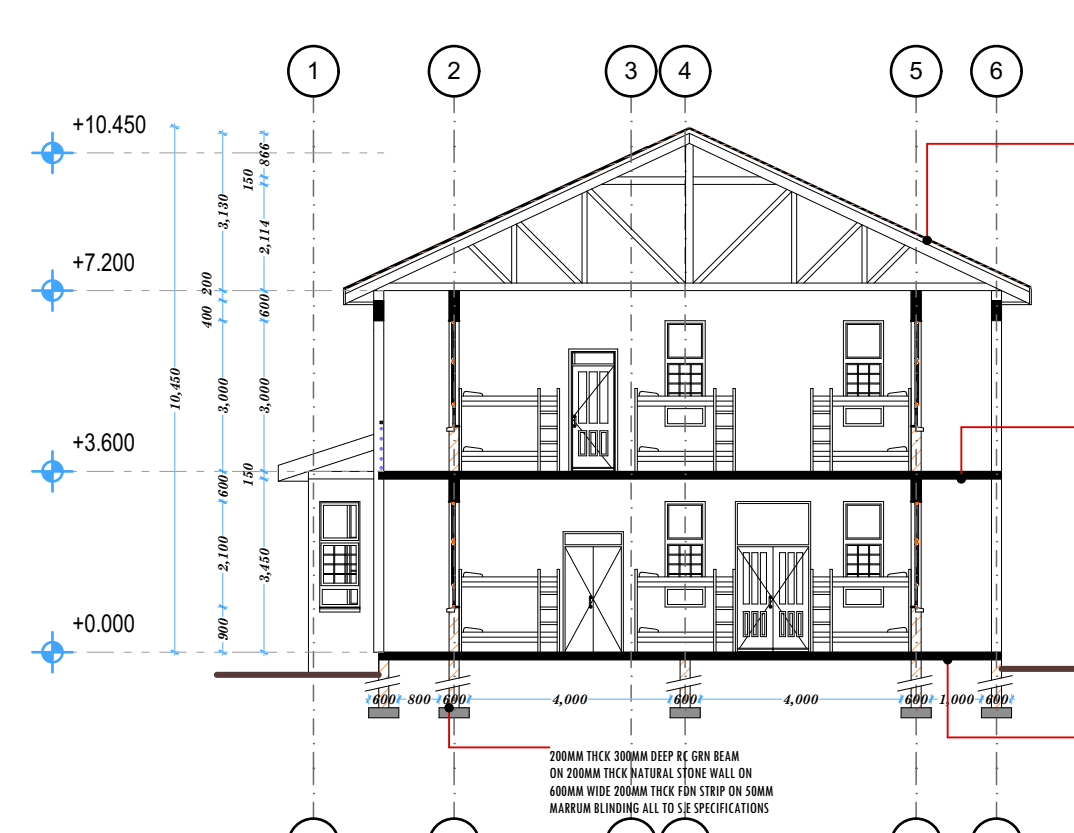
SECTION 01 SCALE 1:100
