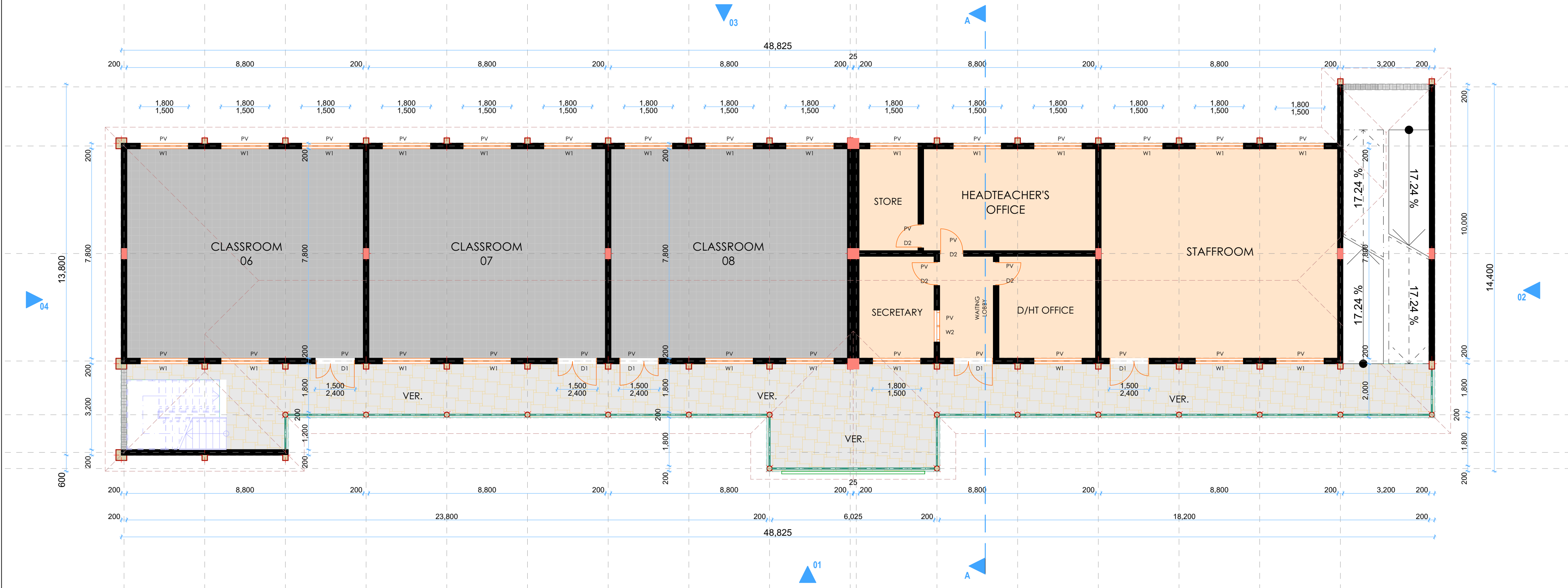
FIRST FLOOR PLAN 1:100
