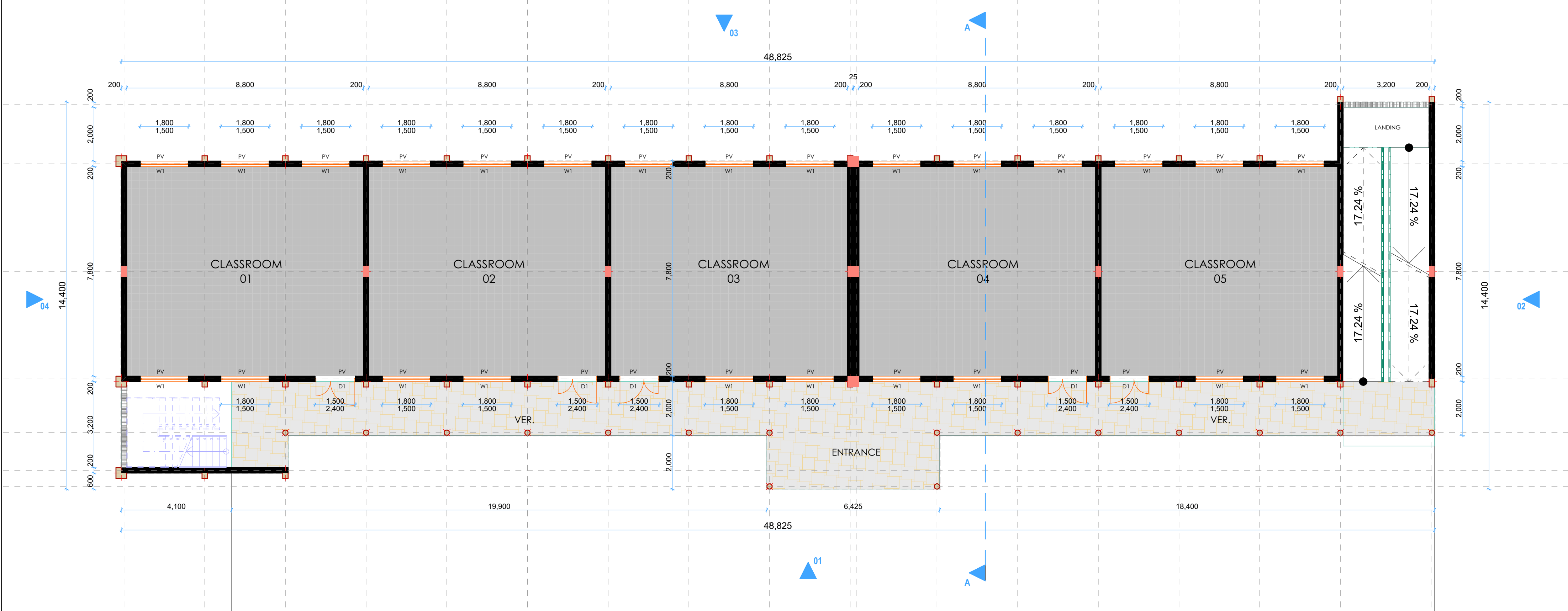
GROUND FLOOR PLAN 1:100
