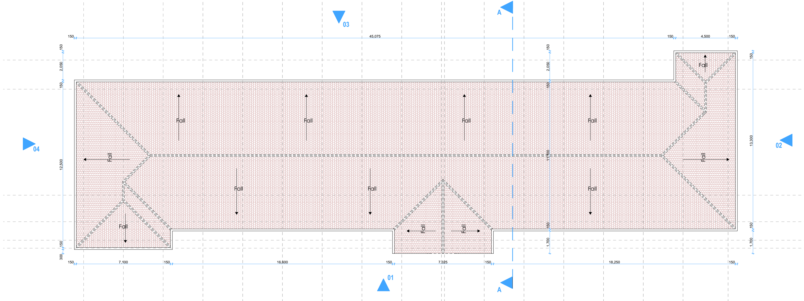
ROOF PLAN 1:150
